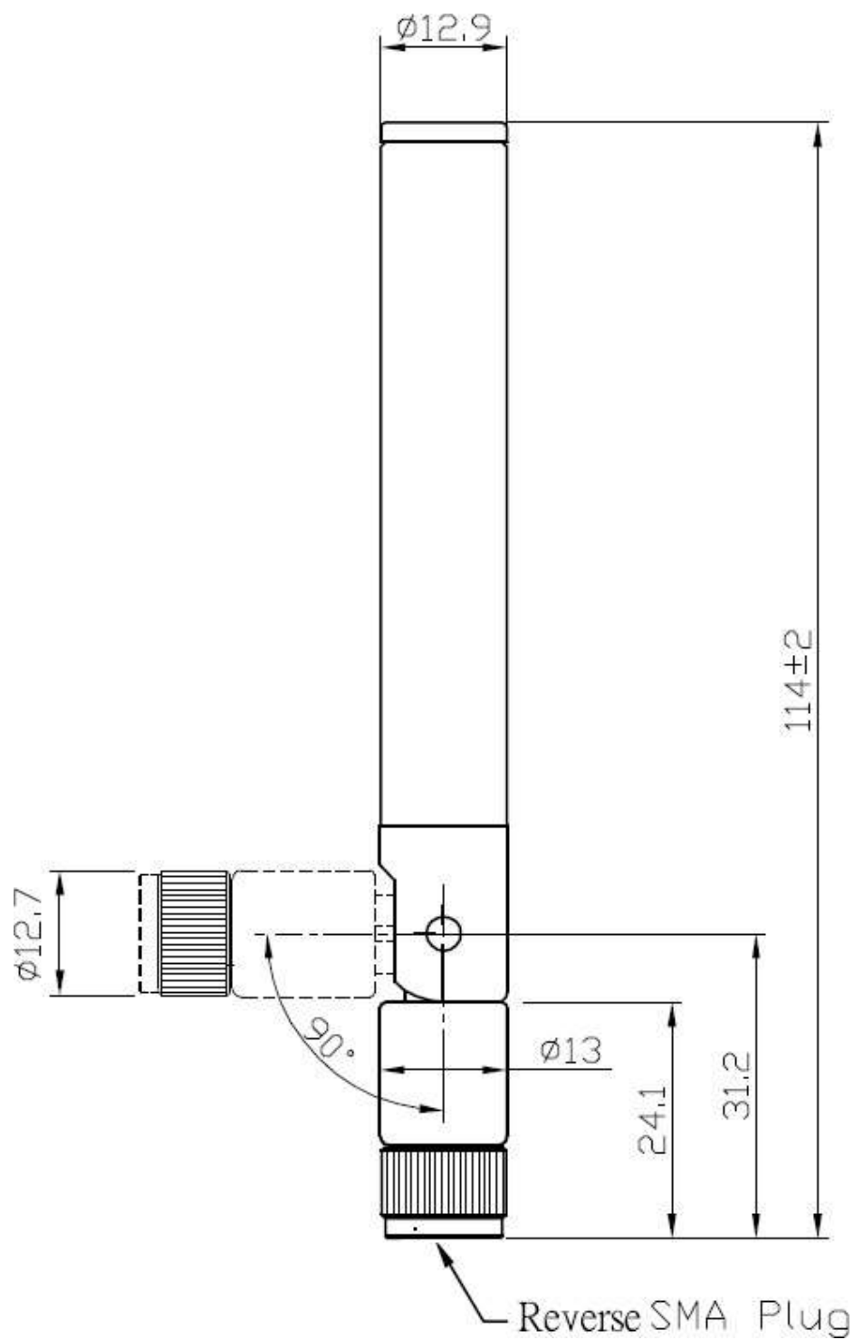
Figure 1 Physical Dimensions
